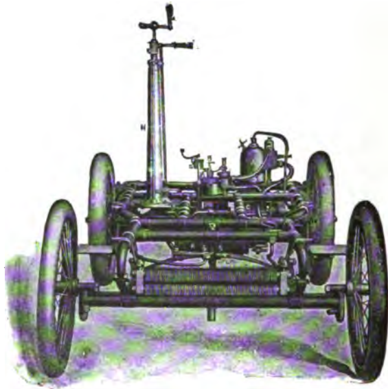
FIG. 386.—Front view of the Running Gear and Mechanism of a Typical De Dion Carriage. A is the motor; B , the vaporizer or carburetter; H , the combined steering and control pillar; I , the variable speed control and brake; J , the steering handle; K , the muffler; L , the radiating coil. This cut shows the relative position of the parts indicated in the last three figures.
